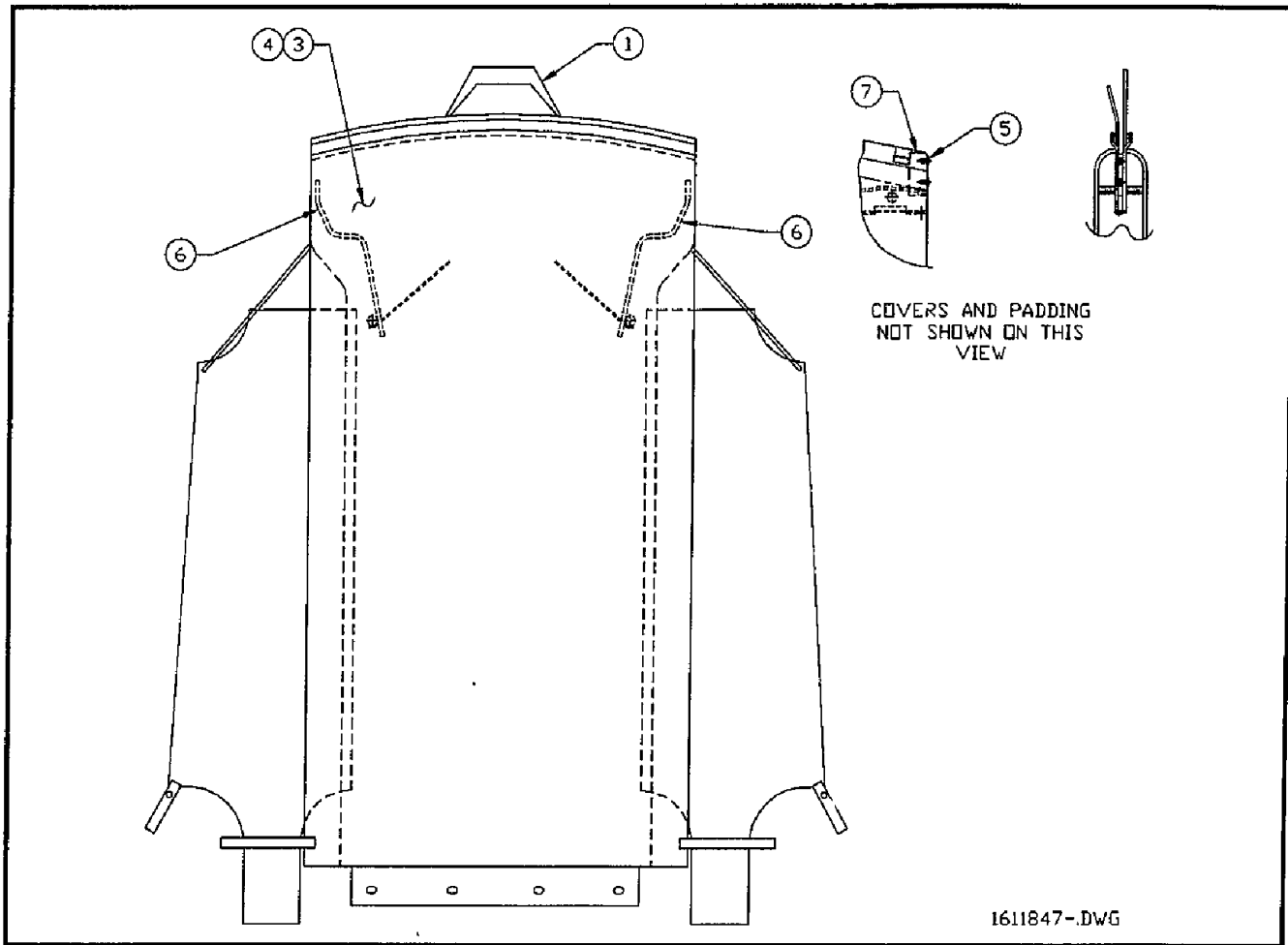
Figure 6-12. Buck Assembly
