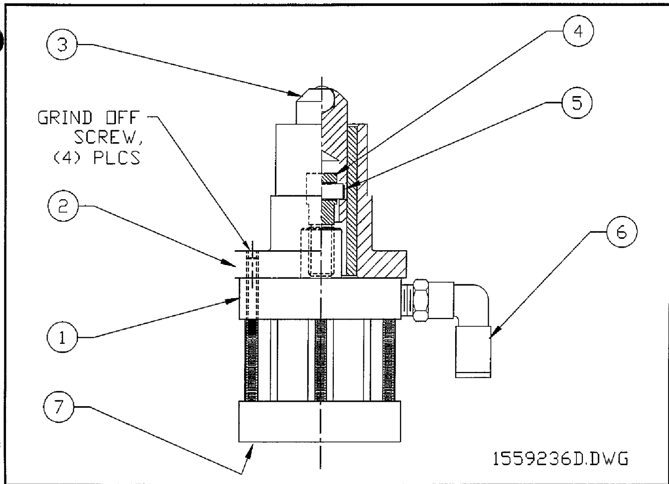
Figure 6-21. Detent Pin Assembly
