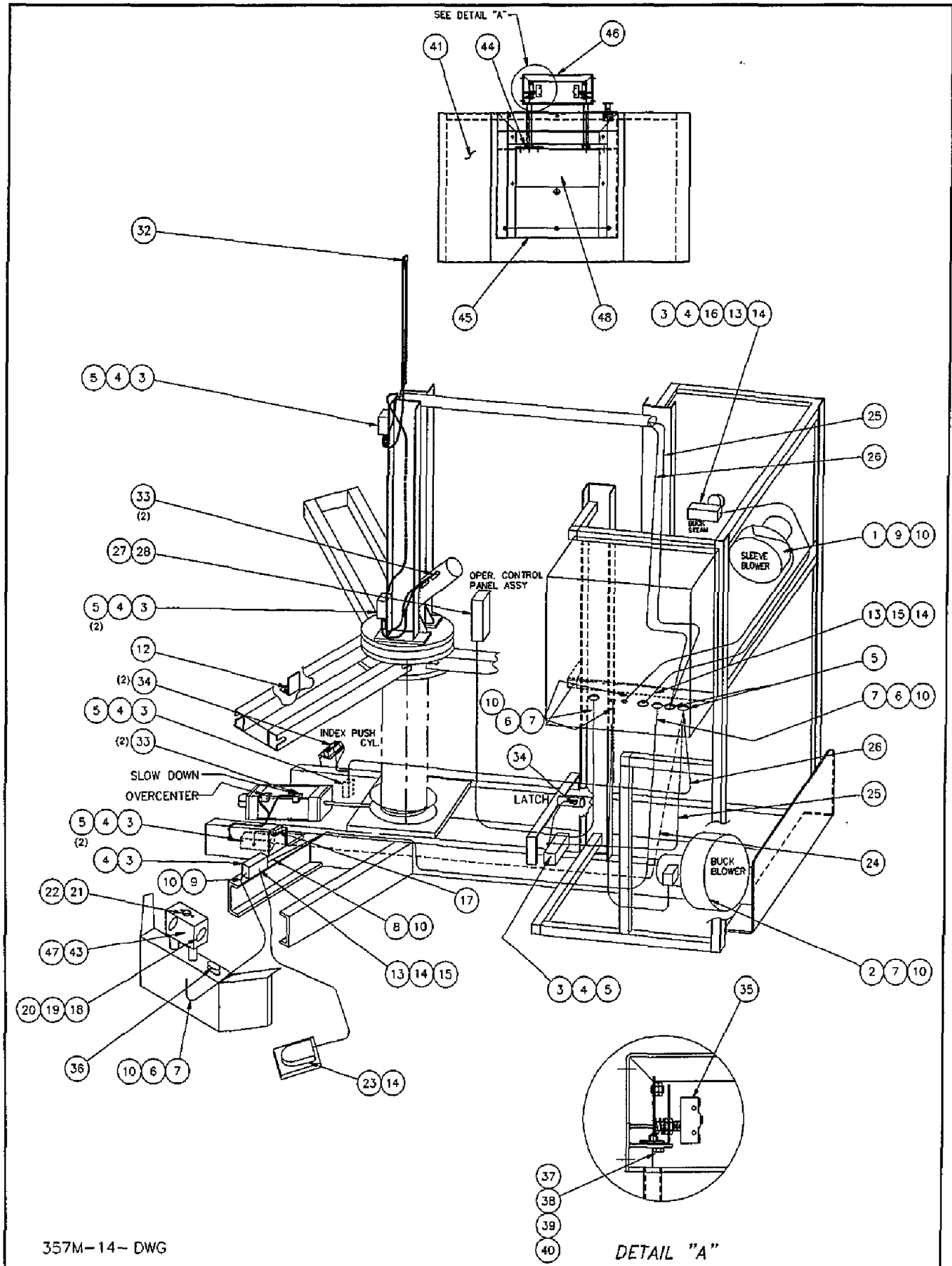
Figure 6-54. Electrical Parts
