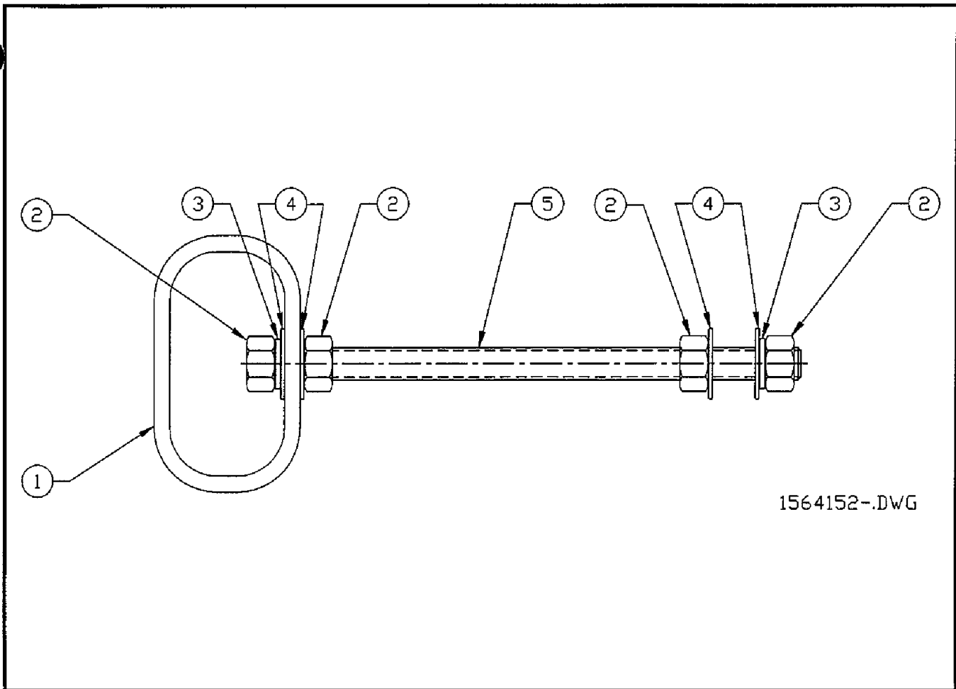
Figure 6-10. Bumper Assembly, Rear Head Stop
