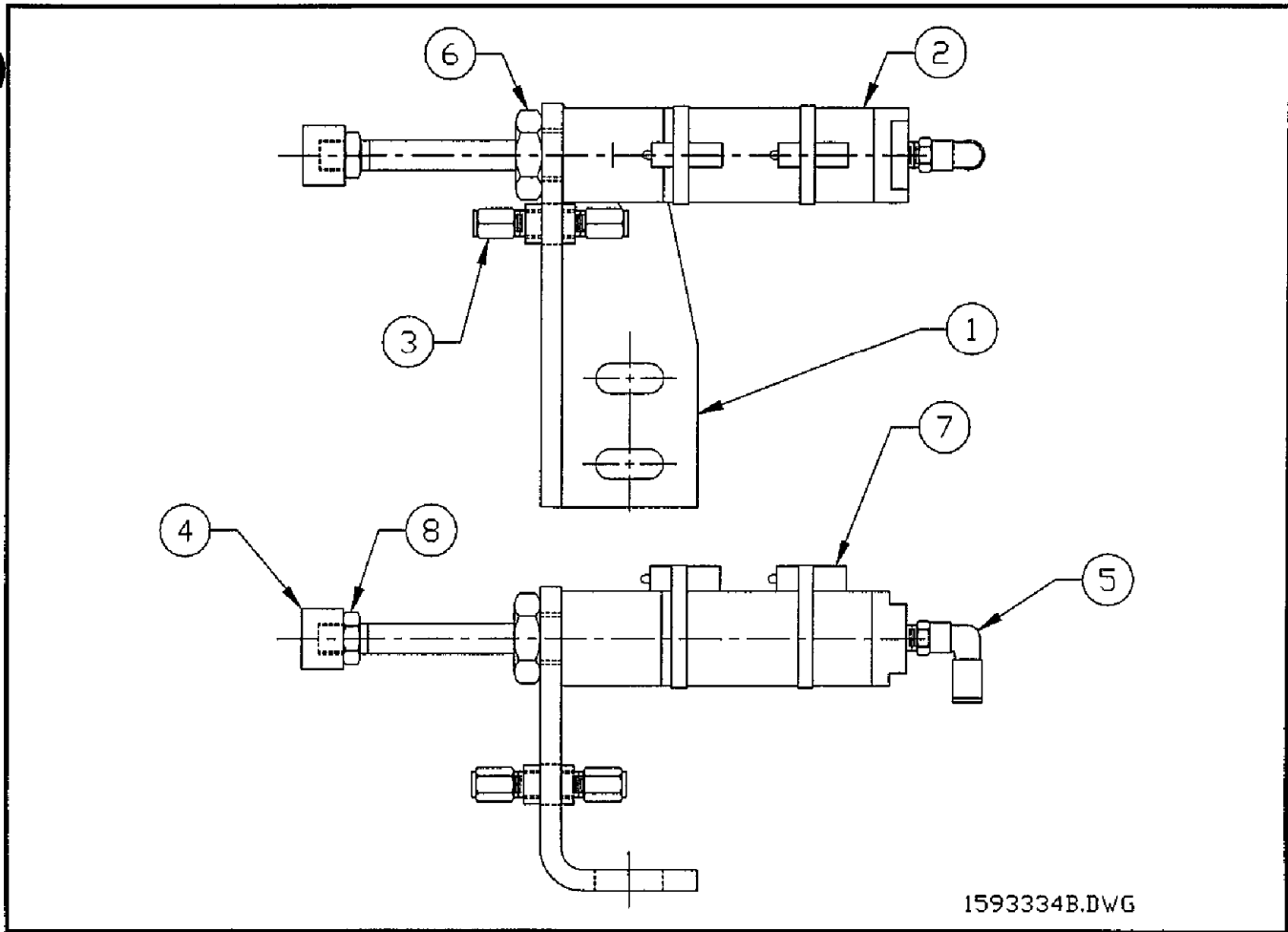
Figure 6-19. Cylinder and Bracket Assembly, Indexing
