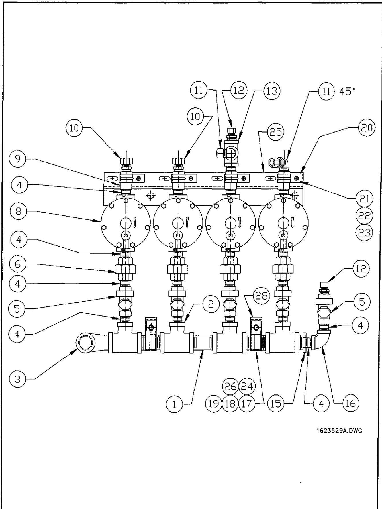
Figure 6-40. Manifold Assembly, Steam
