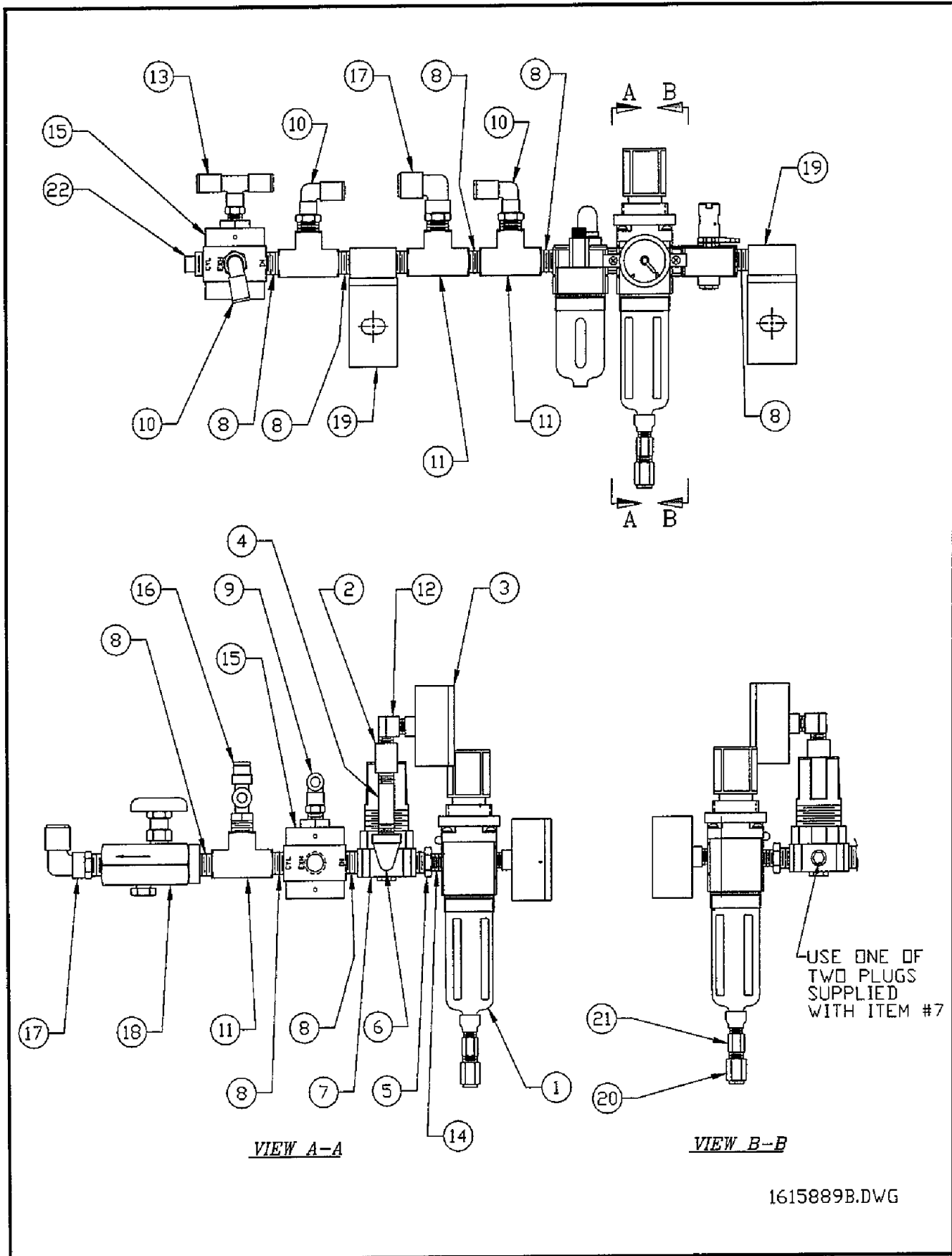
Figure 6-31. Air Inlet Assembly
