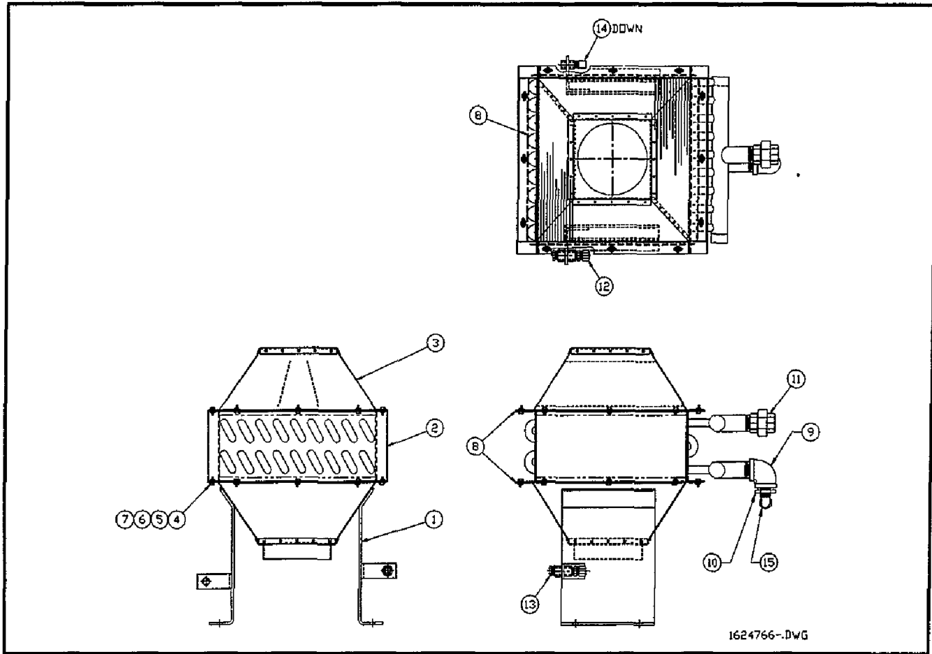
Figure 6-43. Steam Coil
