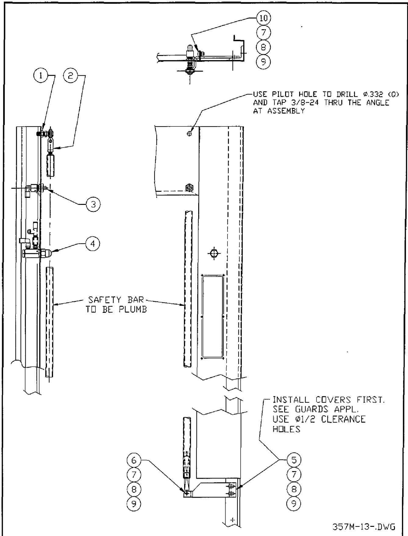
Figure 6-25. Safety Bar Application
