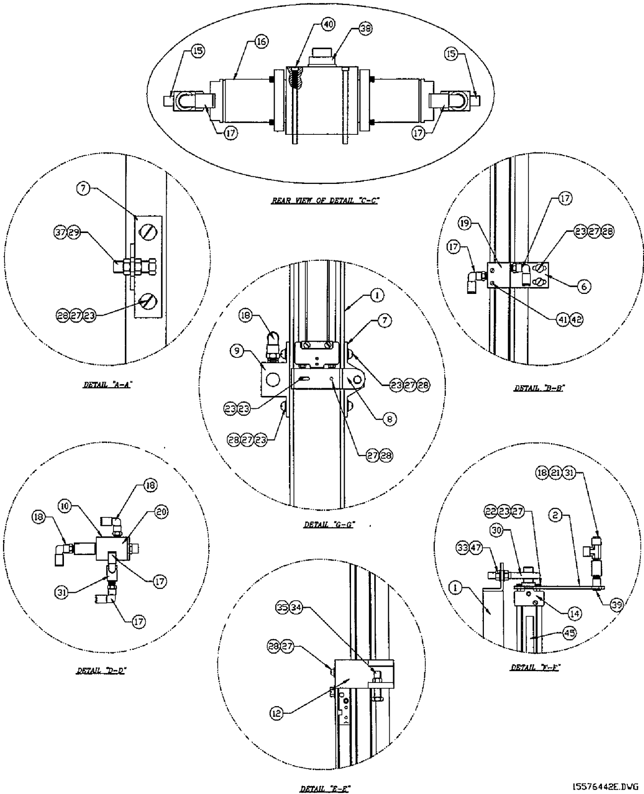
Figure 6-50. Shirt Takeaway Assembly, L.H.. (Sheet 2 of 2)
