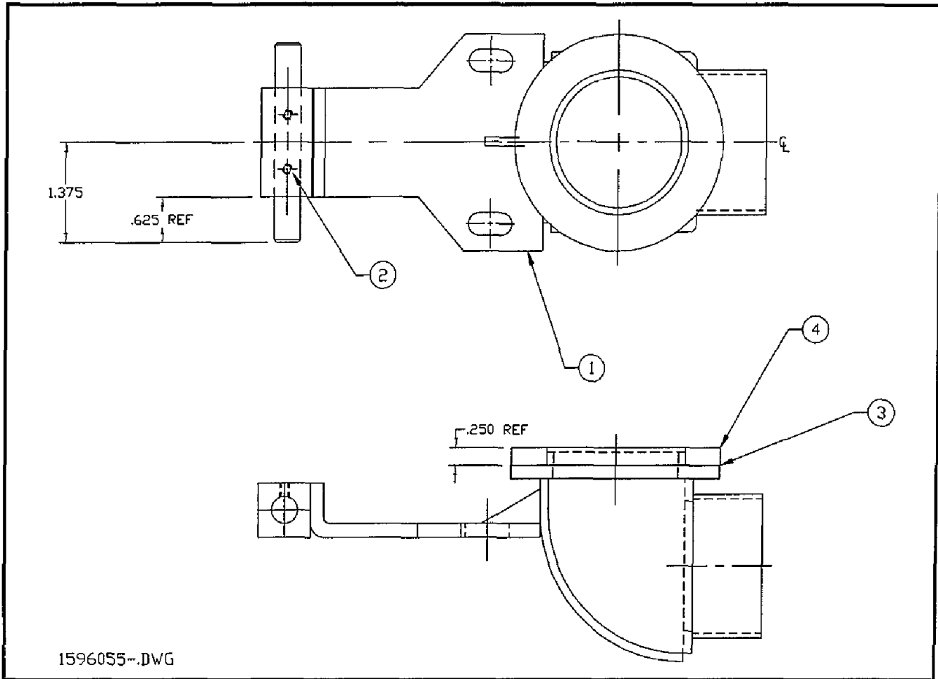
Figure 6-16. Discharge Tube Assembly, Vacuum
