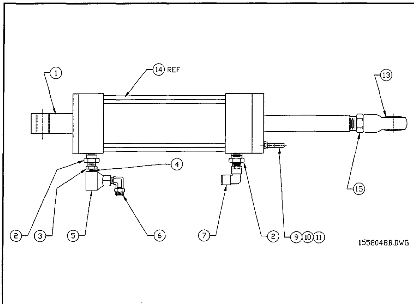
Figure 6-20. Air Cylinder Assembly, Indexing
