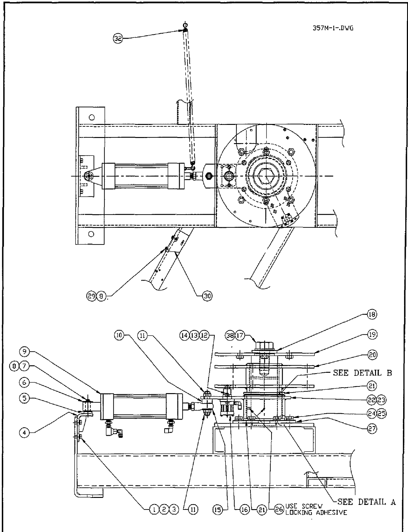
Figure 6-18 Indexing Assembly (sheet 1 of 2)
