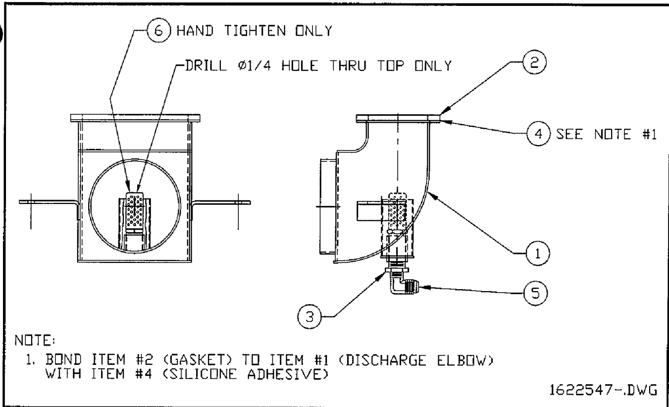
Figure 6-44. Discharge Elbow Assembly
