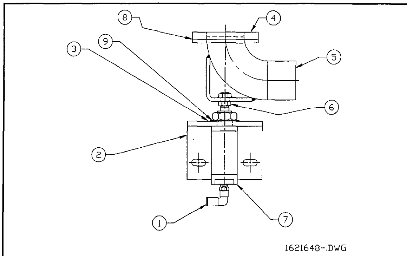
Figure 6-36. Discharge Tube Assembly
