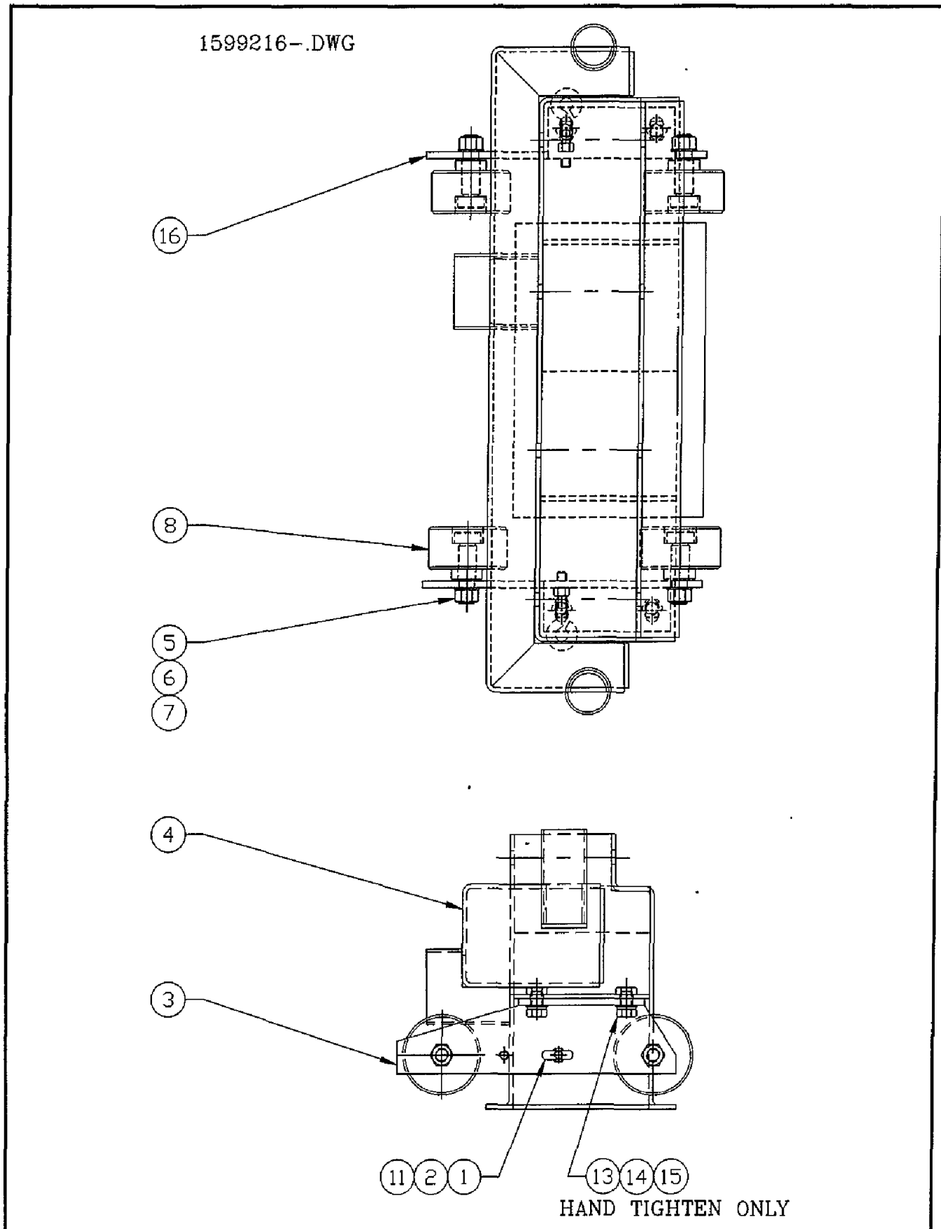
Figure 6-14. Receiving Tube Assembly
