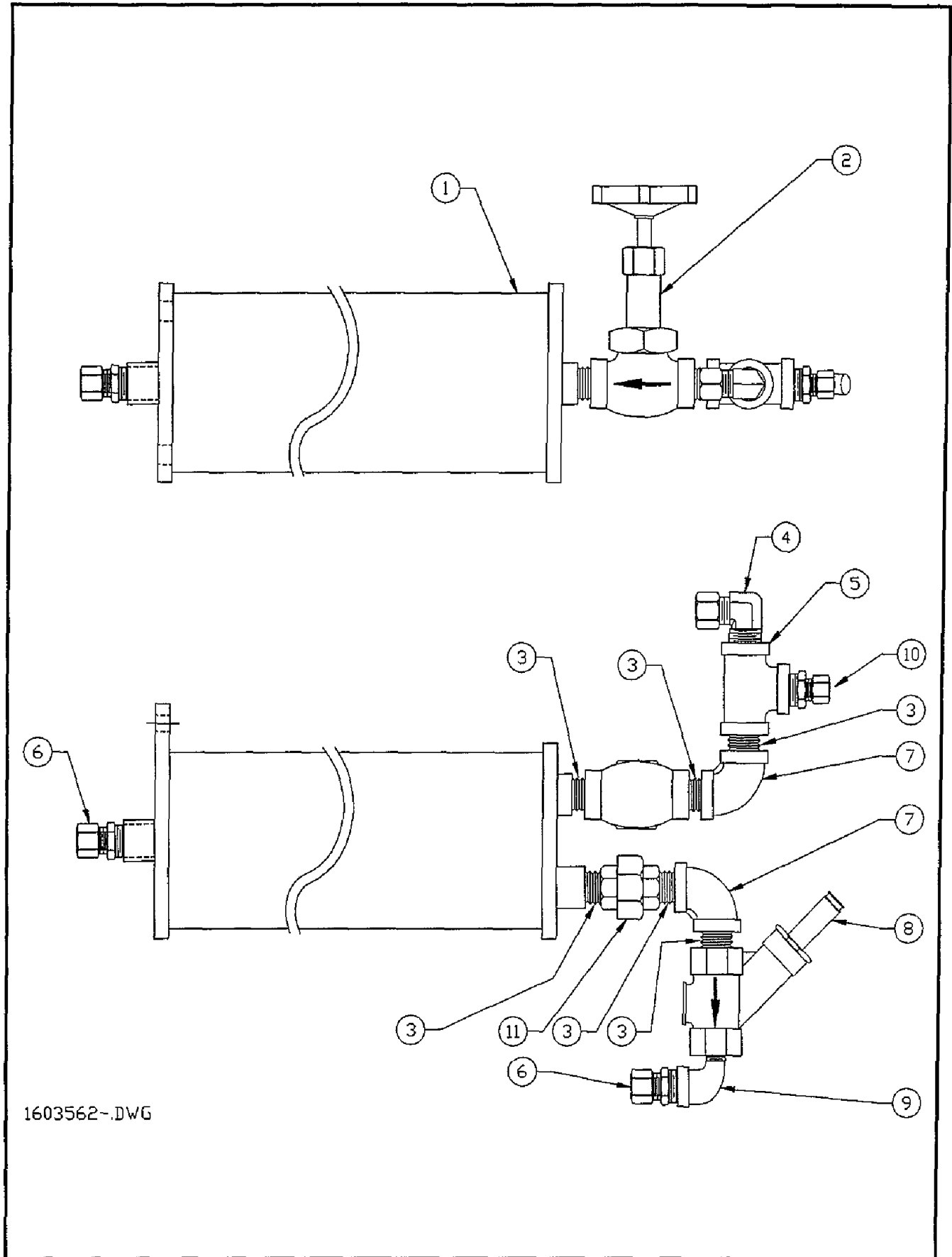
Figure 6-42. Condenser Tank Assembly
