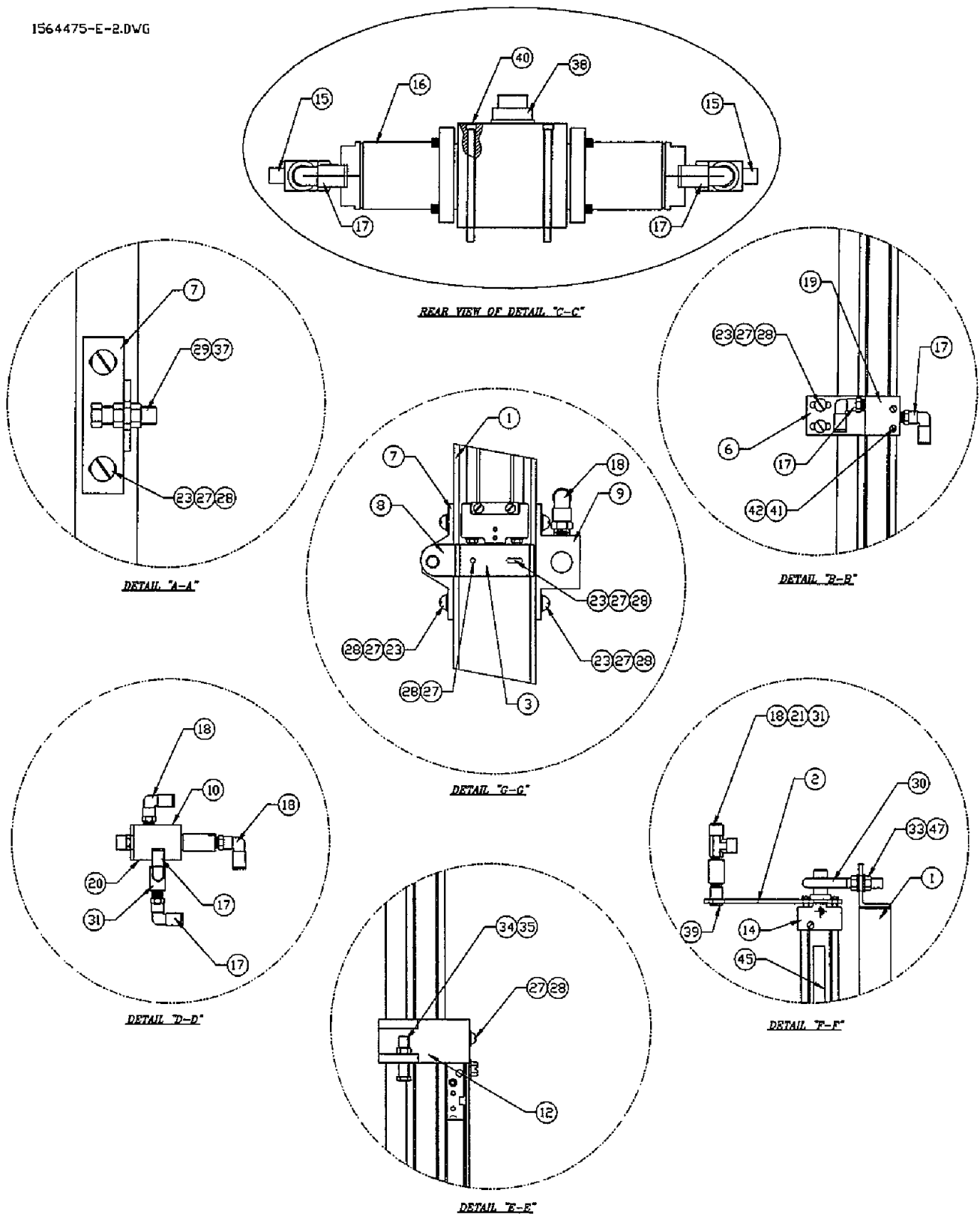
Figure 6-47. Shirt Takeaway Assembly, R.H. (Sheet 2 of 2)
