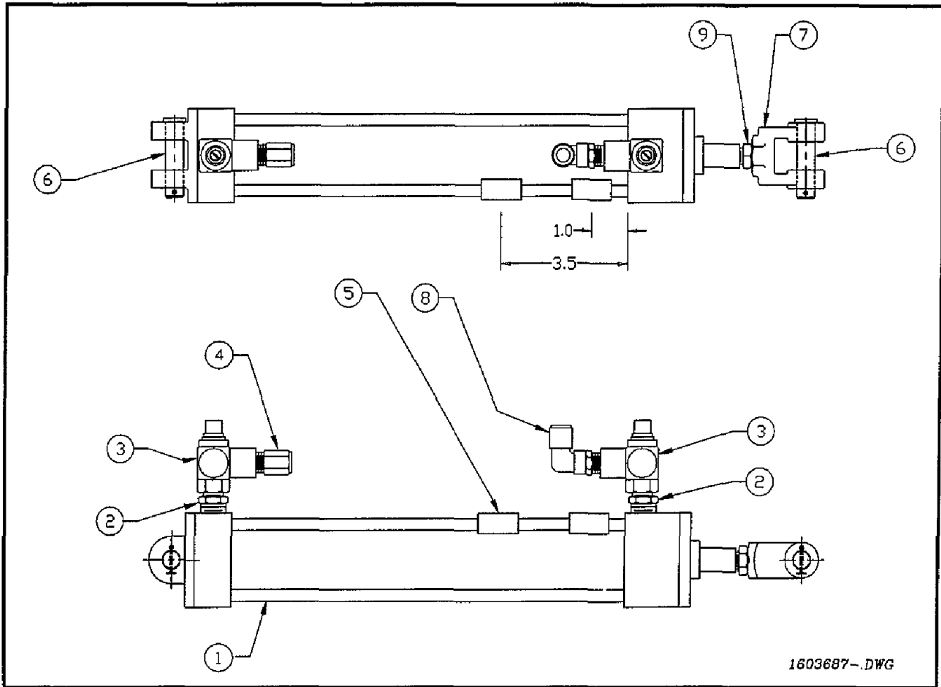
Figure 6-7. Cylinder Assembly, Head Closing
