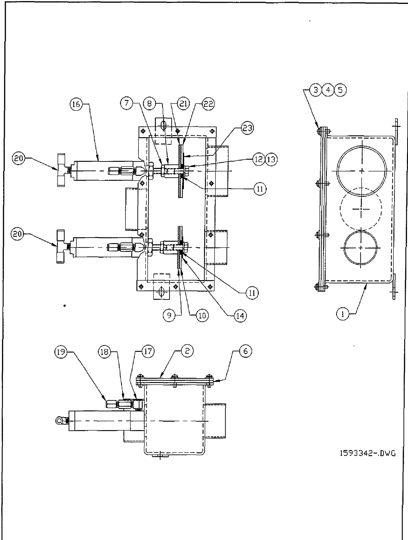
Figure 6-38. Damper Box Assembly, Heat Exchanger
