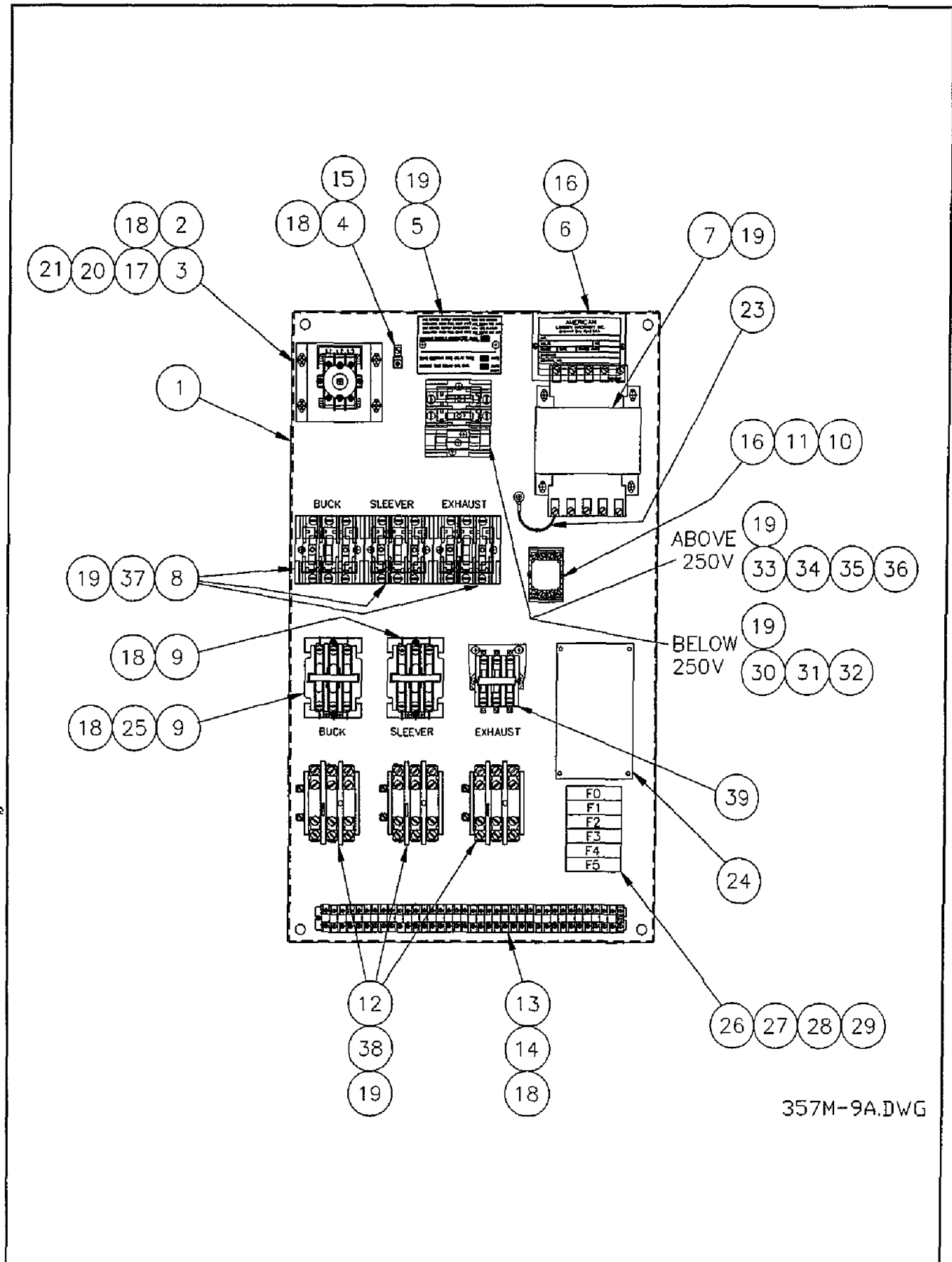
Figure 6-52. Control Panel Assembly
