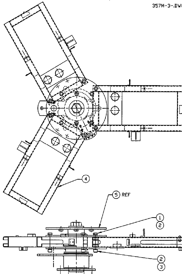
Figure 6-17. Buck Support Assembly
