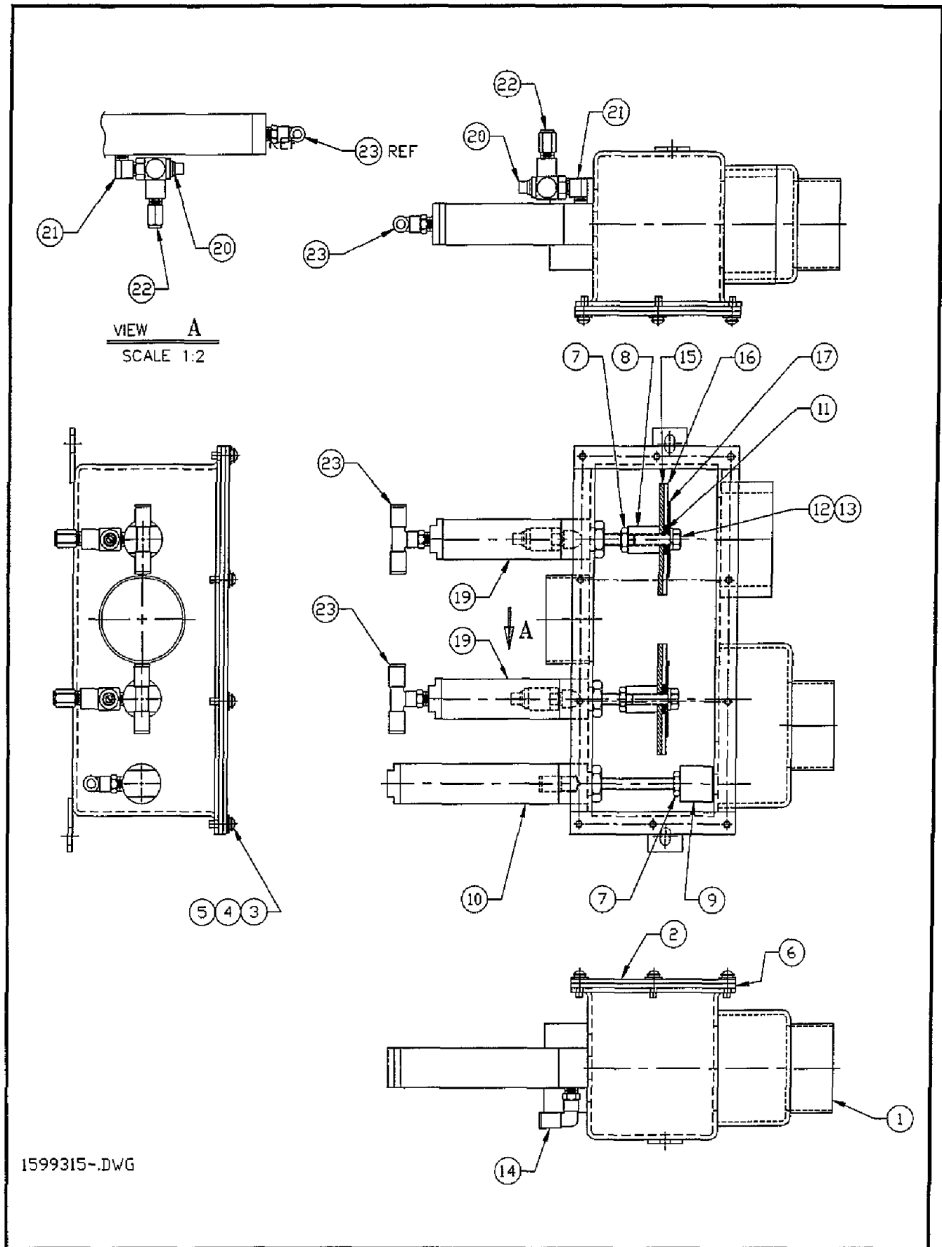
Figure 6-34. Damper Box Assembly, Blower
