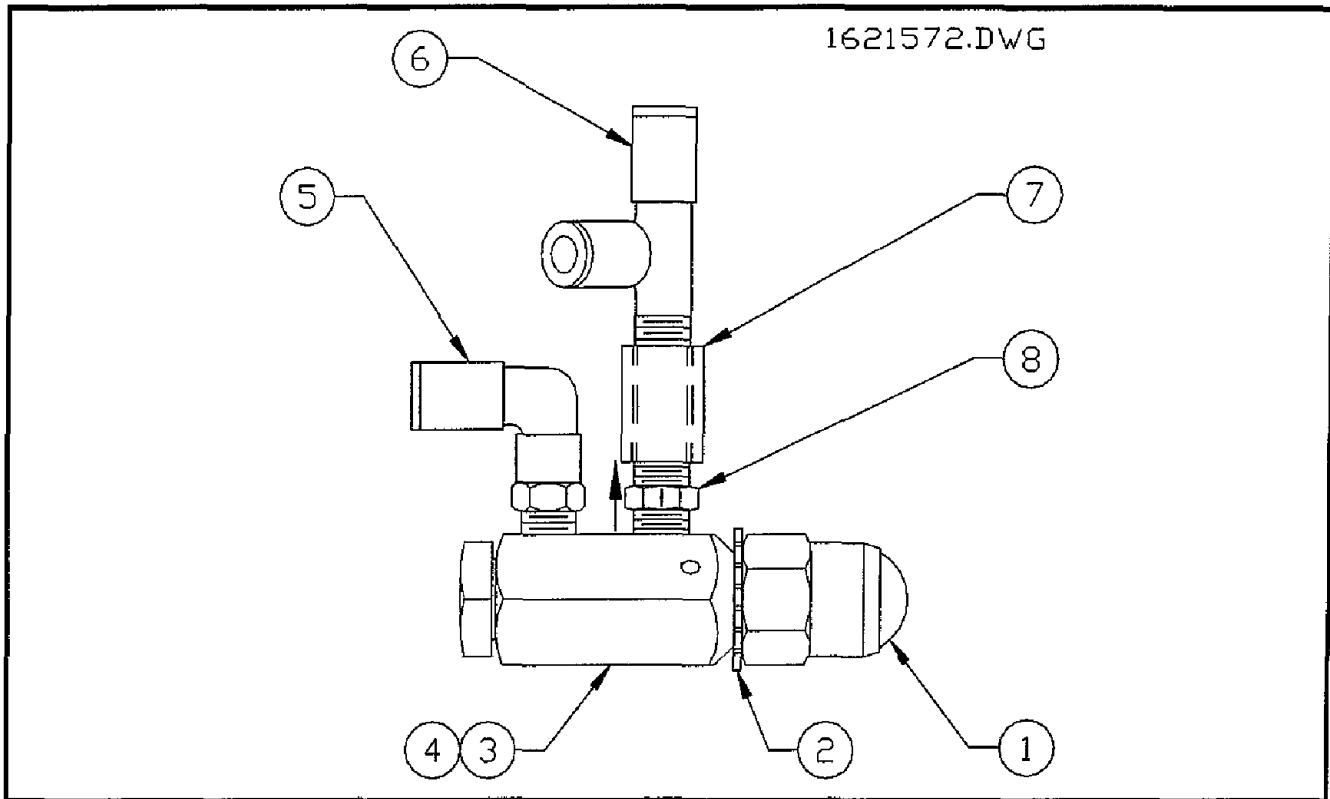
Figure 6-28. Valve Assembly Reset
