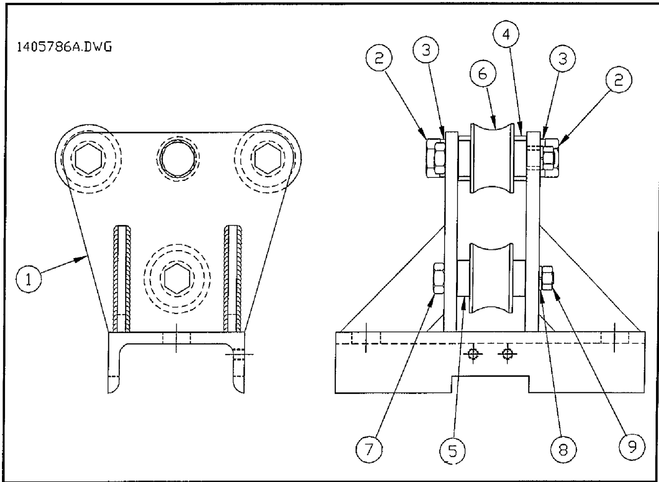
Figure 6-9. Roller Bracket Assembly
