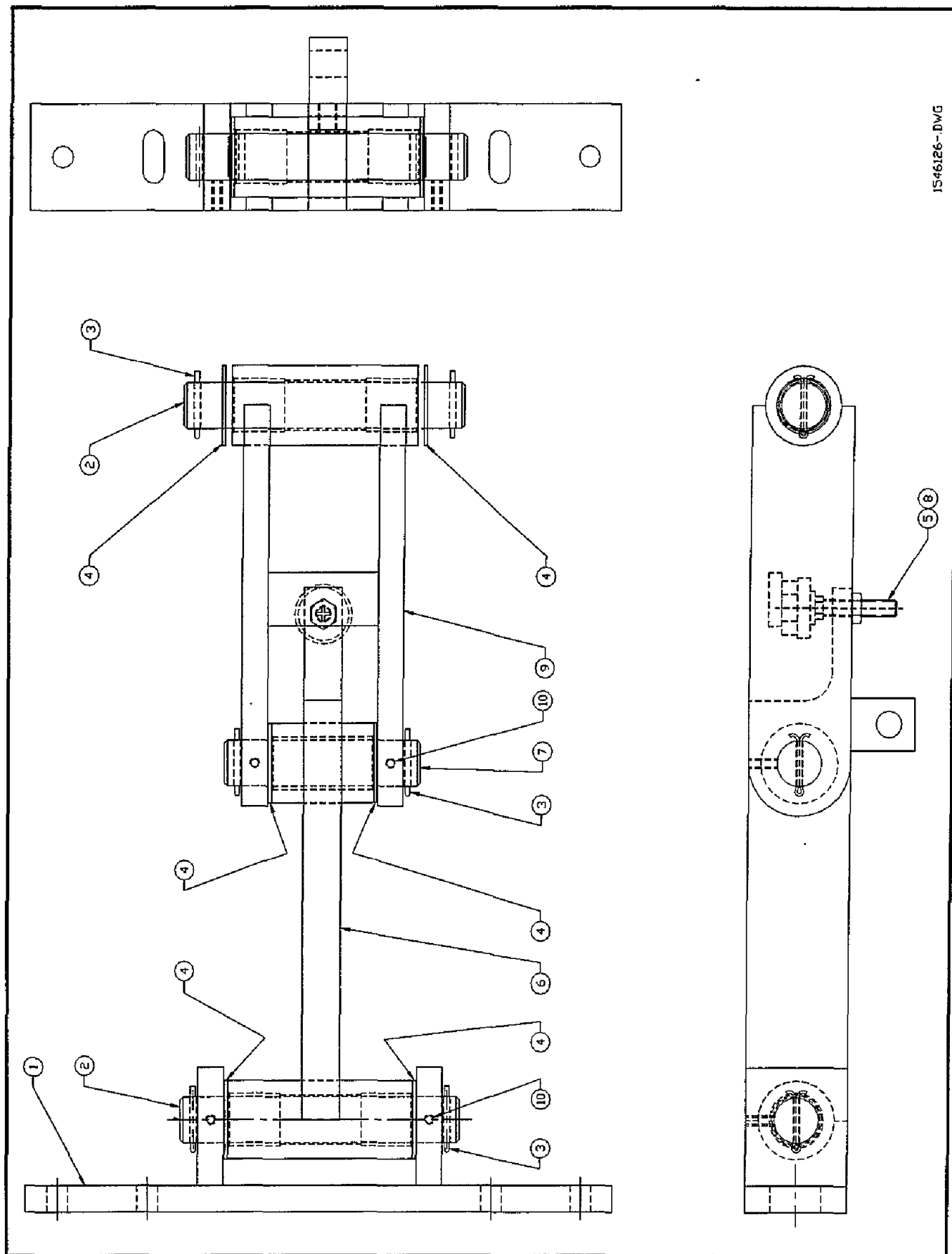
Figure 6-8. Linkage Assembly
