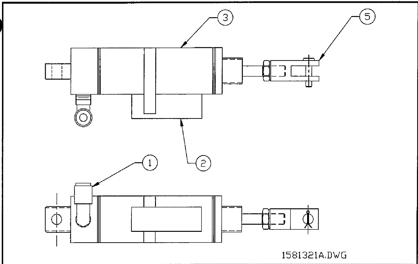
Figure 6-24. Locking Plate Cylinder Assembly
