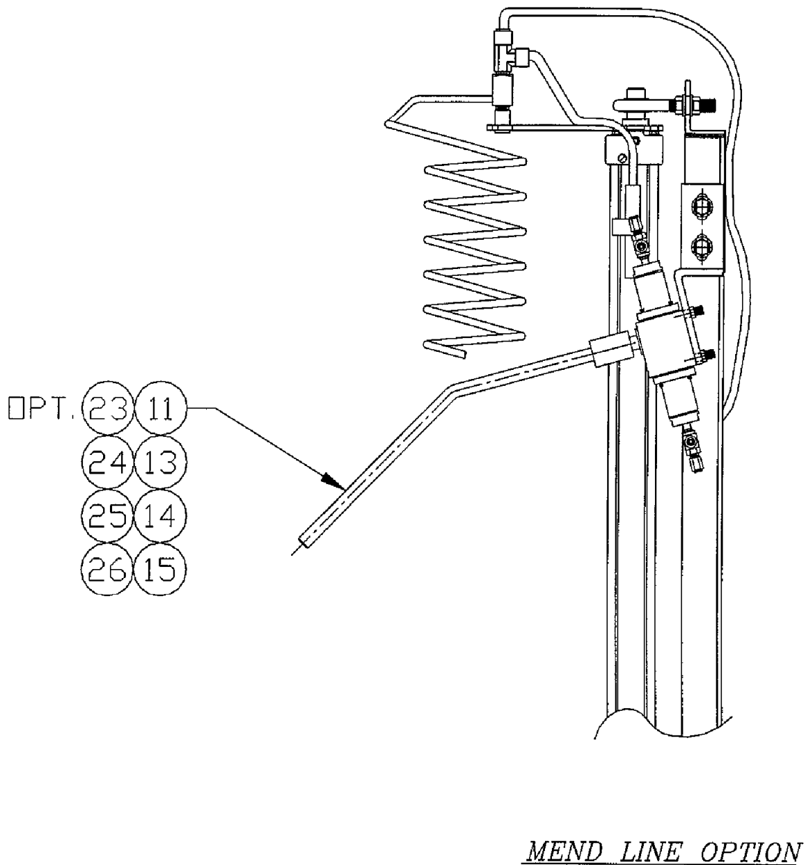
Figure 6-45. Mend Line Option, Right Hand (Sheet 2 of 2)
