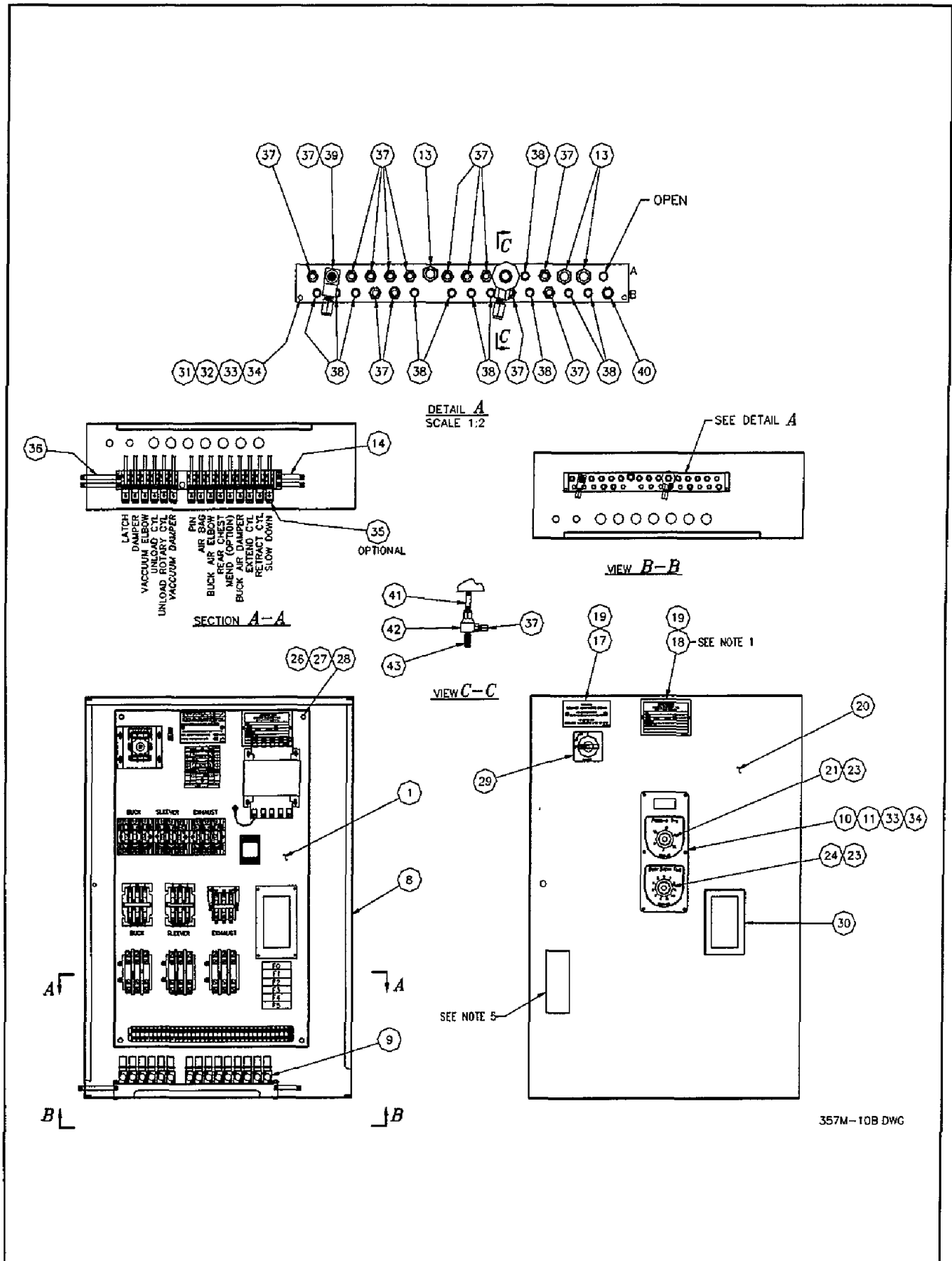
Figure 6-51. Control Assembly
