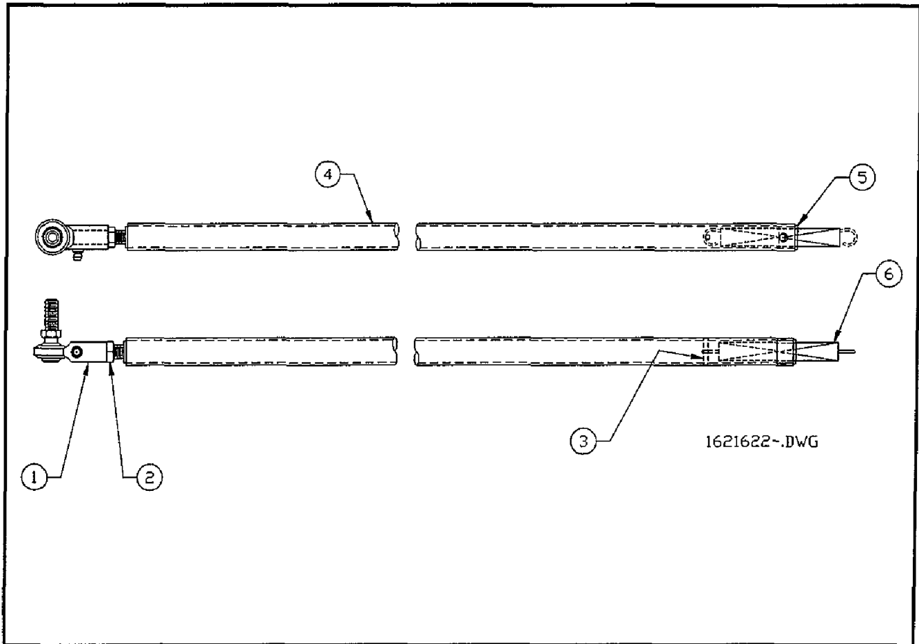
Figure 6-26. Safety Bar Assembly
