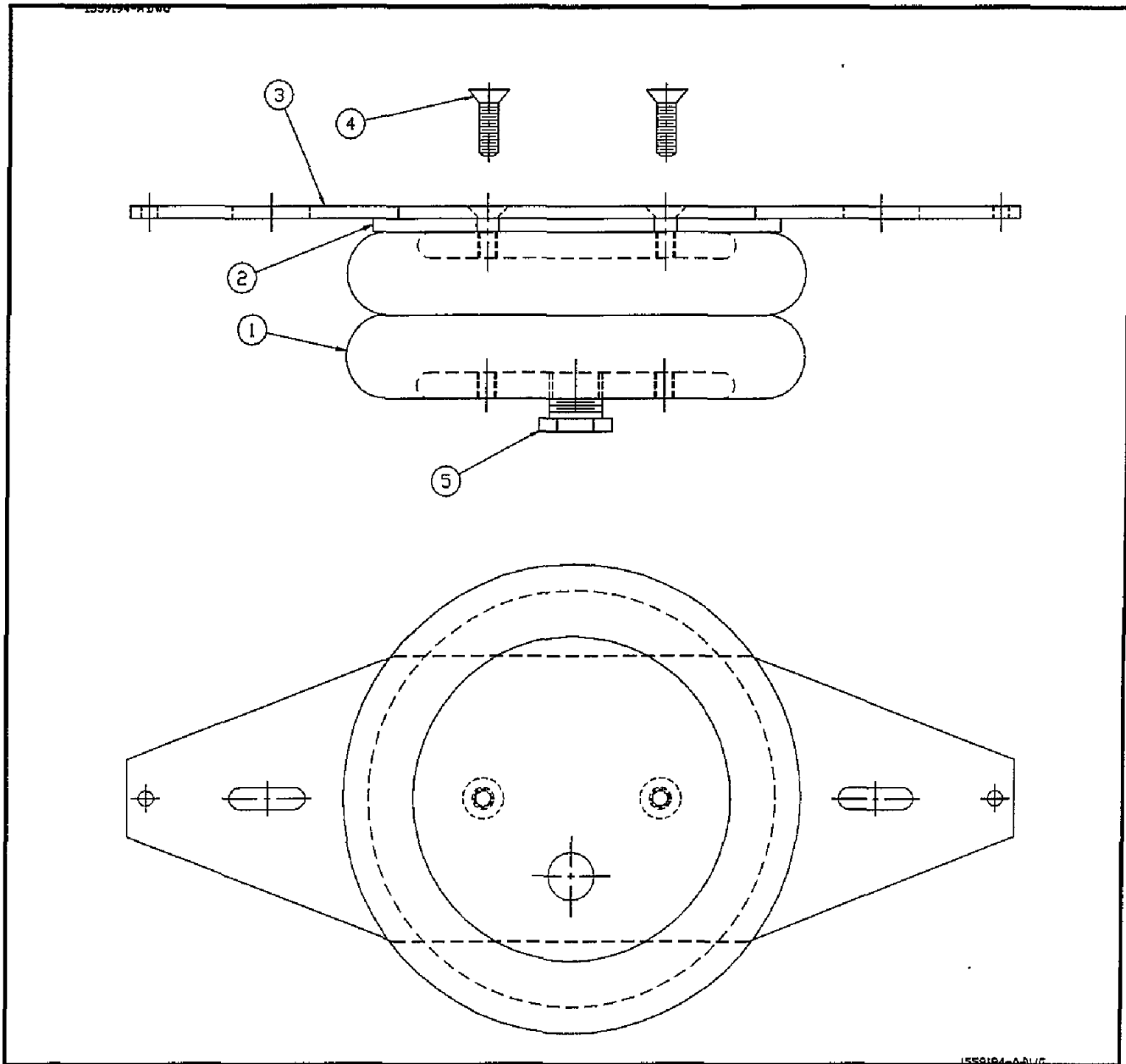
Figure 6-30. Air Bag Assembly
