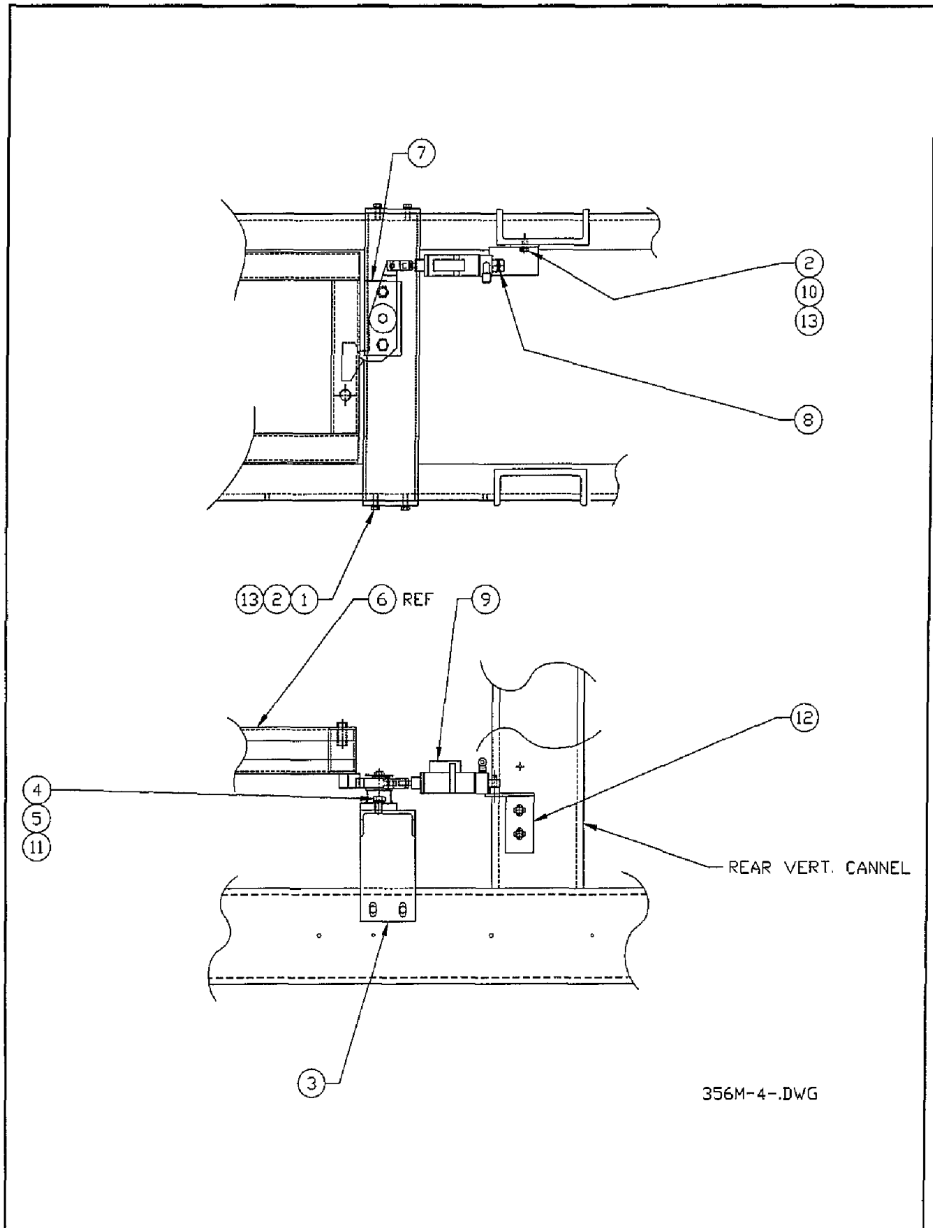
Figure 6-22. Buck Locking Assembly
