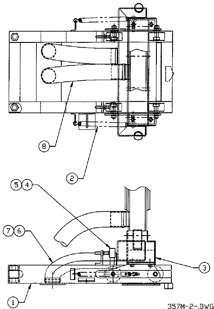
Figure 6-13. Buck Frame Subassembly
