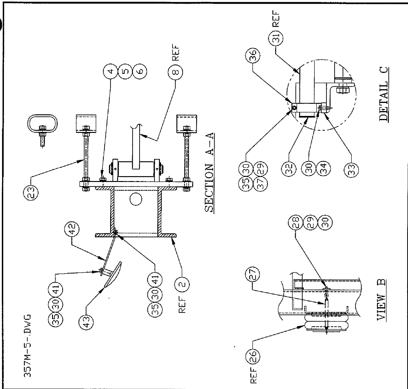
Figure 6-4. Head Closing Assembly (Sheet 2 of 2)
