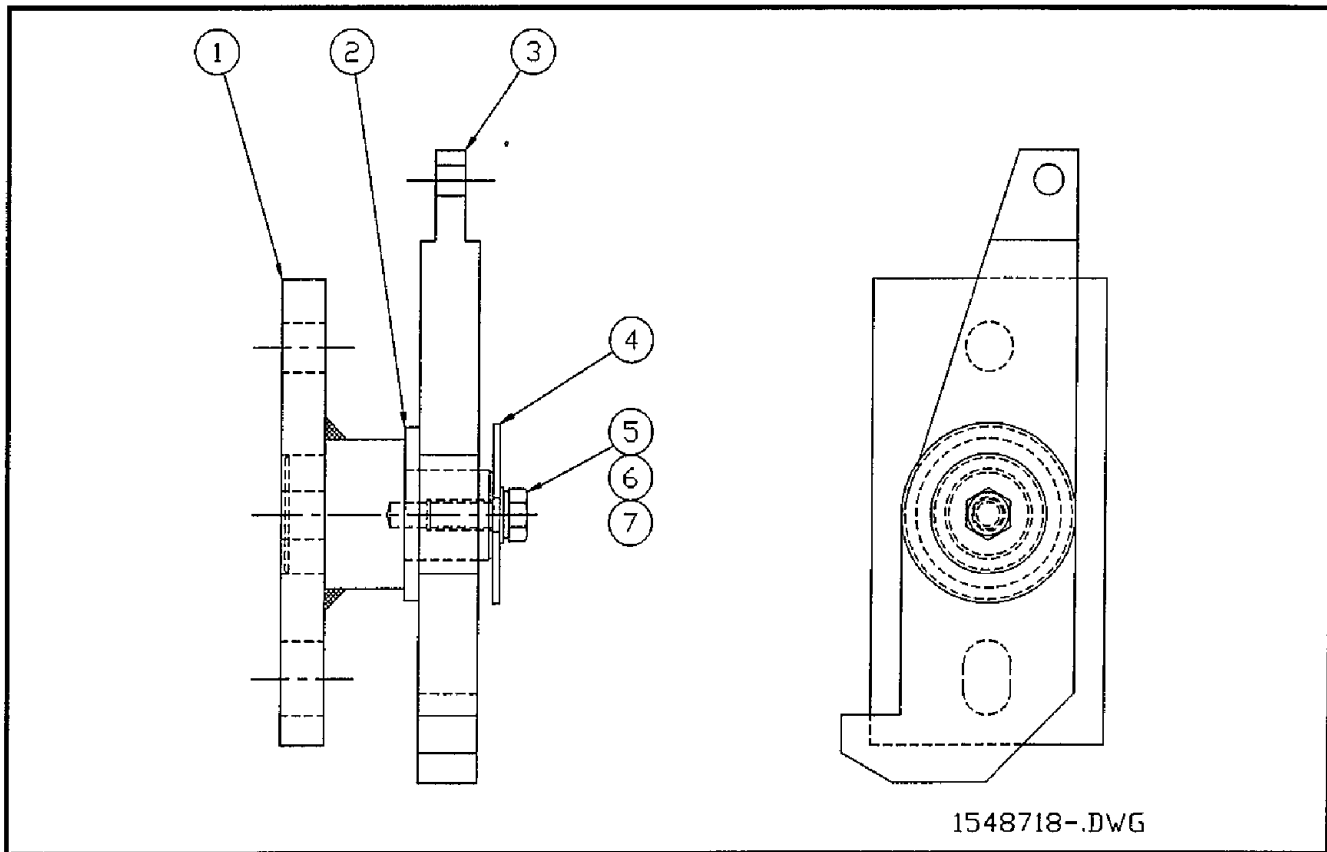
Figure 6-23. Locking Plate Assembly
