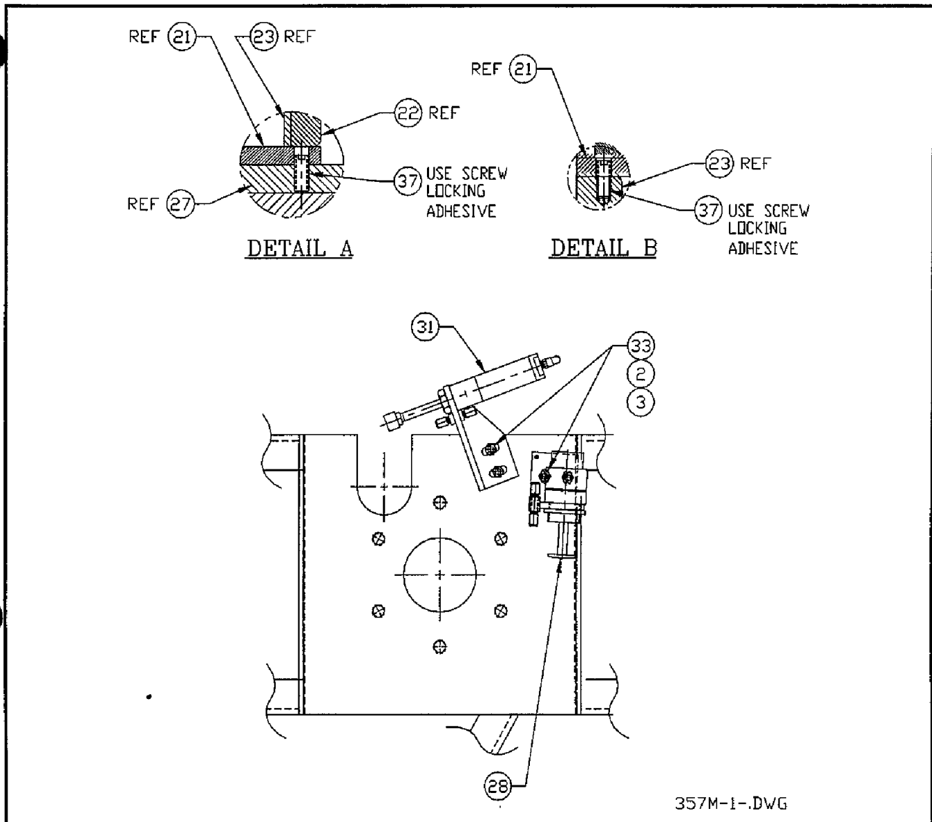
Figure 6-18 Indexing Assembly (sheet 2 of 2)
