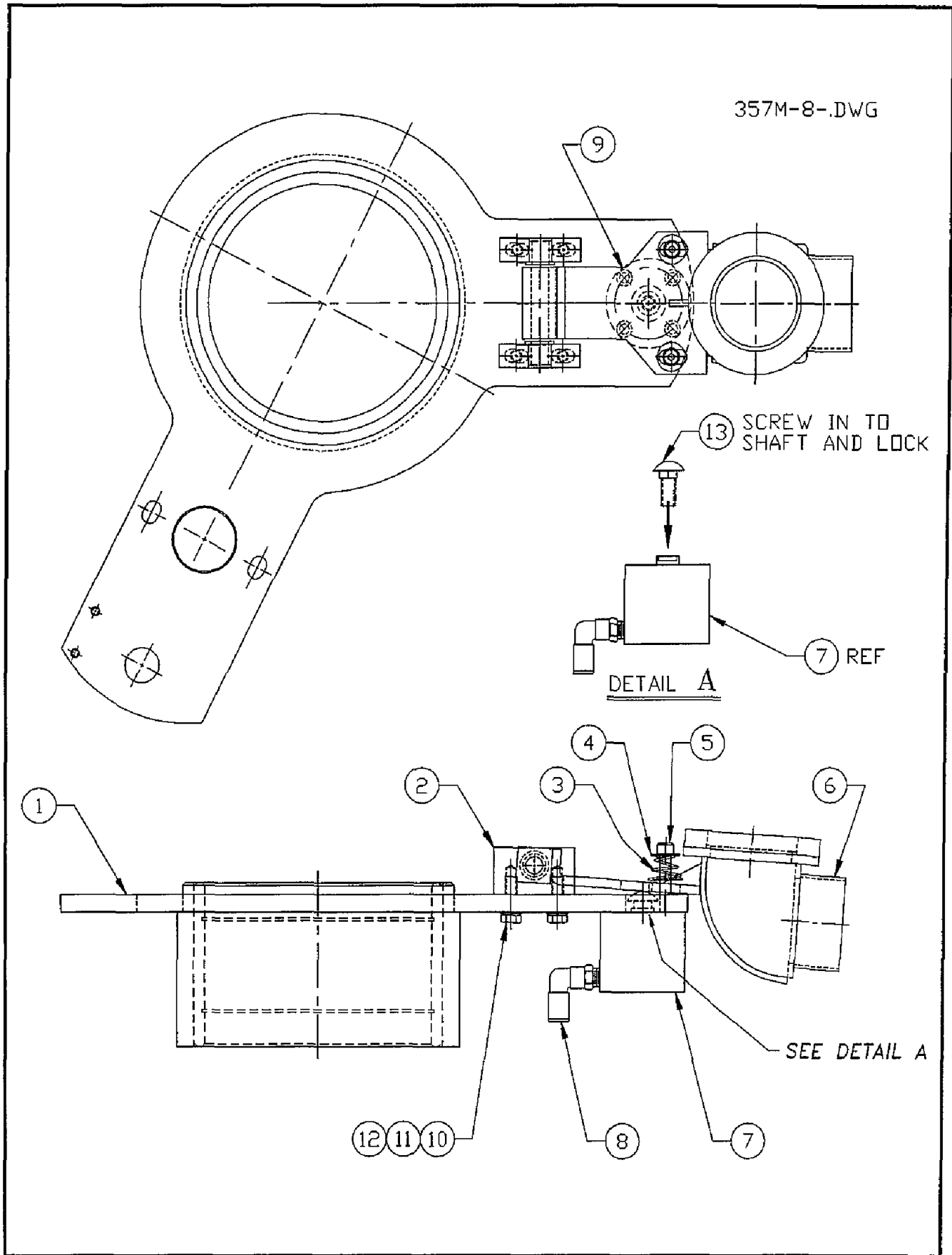
Figure 6-15. Vacuum Assembly
