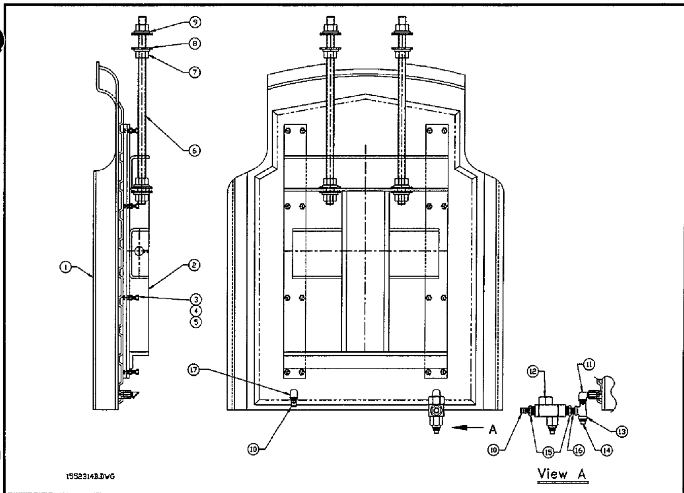
Figure 6-6. Rear Head Assembly
